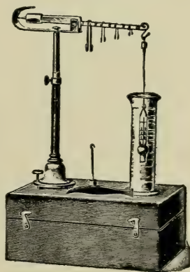
Courtesy of Eimer & Amend. FIG. 154.—Westphal Balance.
